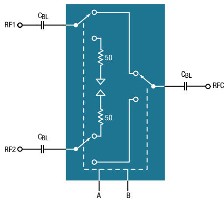
Functional Diagram
