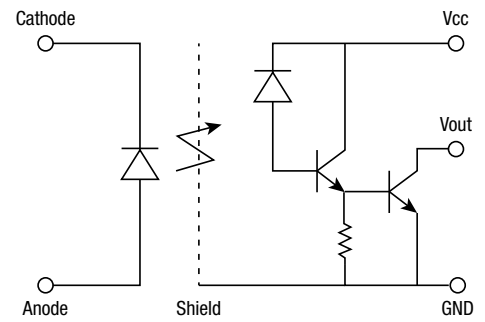
Low Input Current Photodarlington Optocoupler Functional Schematic
