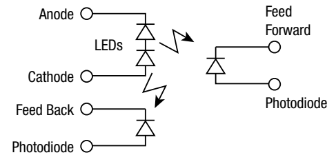
Linear Optocoupler Functional Schematic
